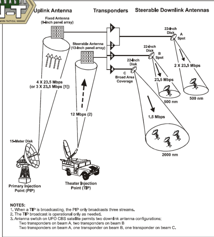
Figure 4-11. GBS Broadcasting Architecture
